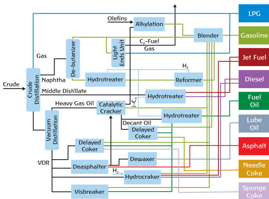
Figure A1.6 ● Operation of a Typical Refinery
