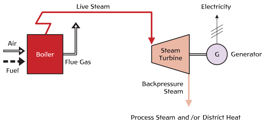
Figure A1.1 ● Backpressure Power Plants
