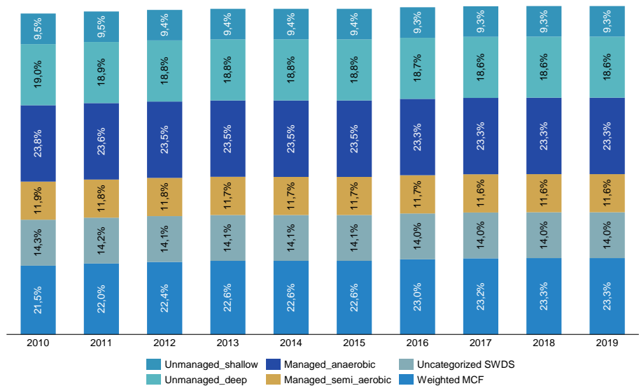
Figure 118. Methane correction factor in industry
