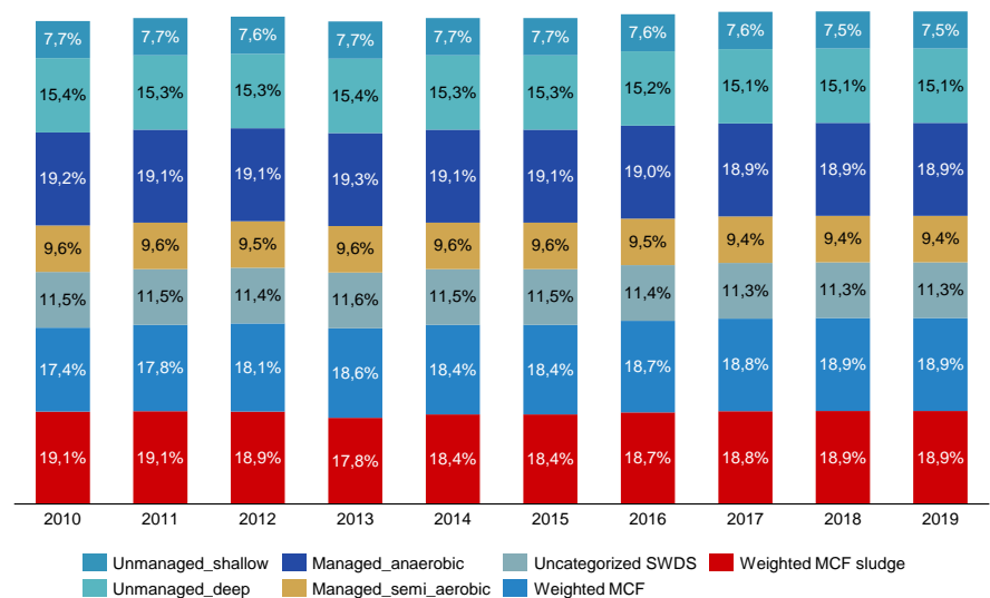
Figure 117. Methane correction factor in MSW
