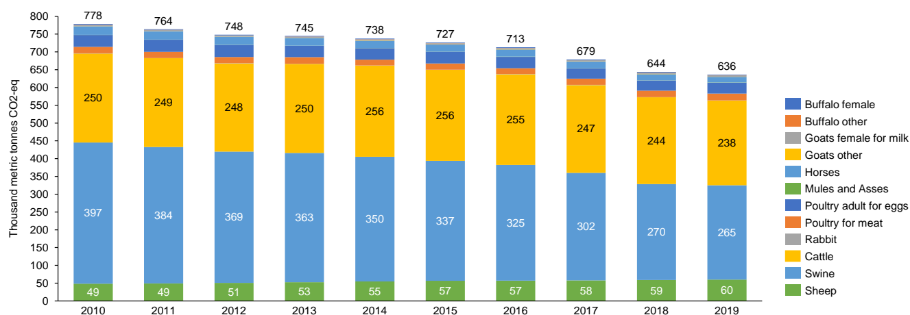
Figure 109. GHG emissions – Manure management (Methane)
