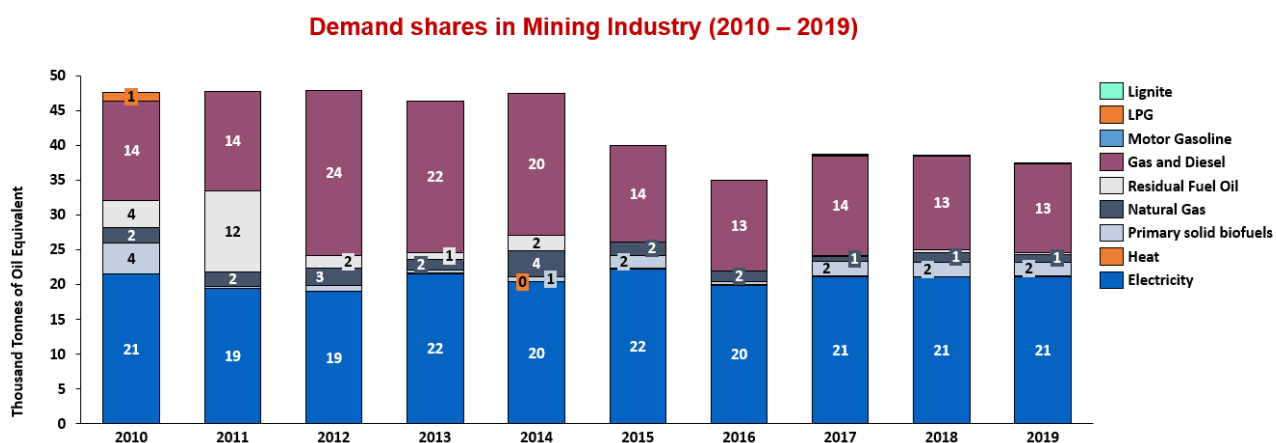
Figure 94. Final energy consumption - Mining
